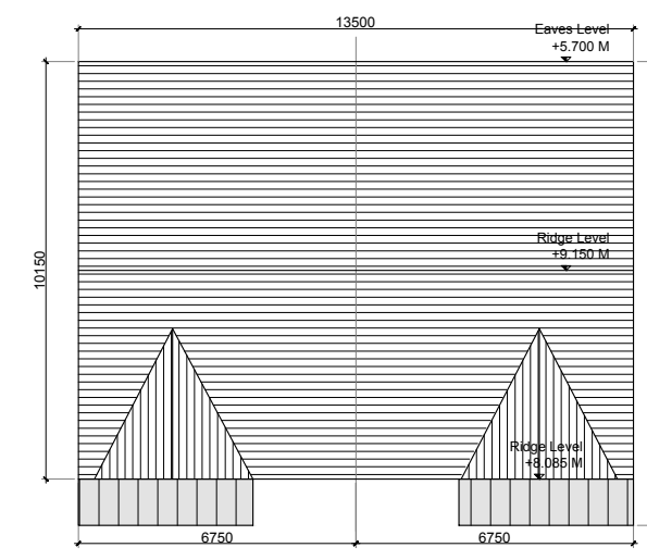
Roof Plan 1:200
