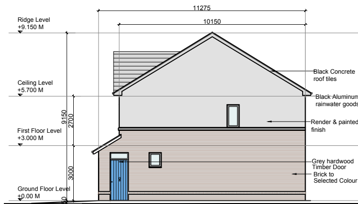
Side Elevation 1:200
