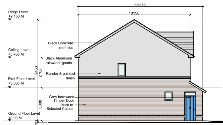
Side Elevation 1:200
