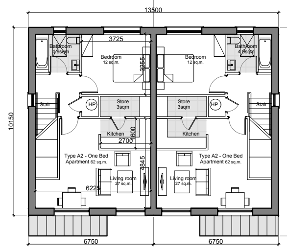
First Floor Plan 1:200
