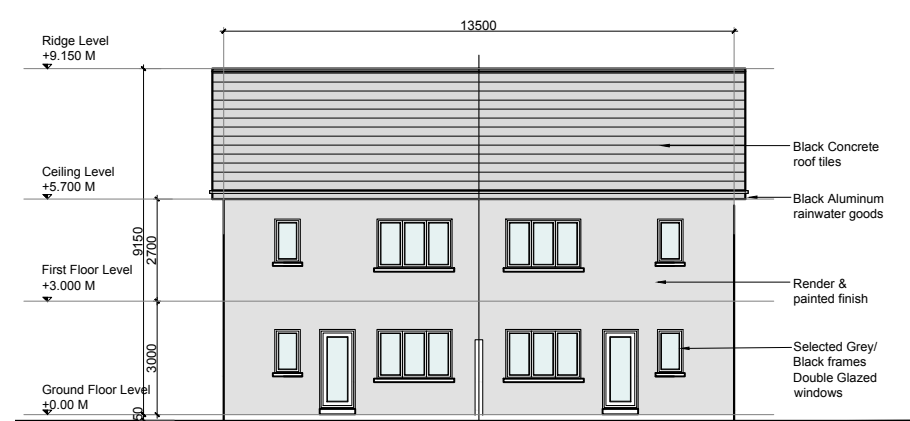
Rear Elevation 1:200
